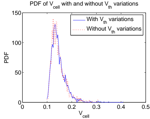
Figure 5.8: PDF of the V_{cell} distribution with and without V_{th} variations
